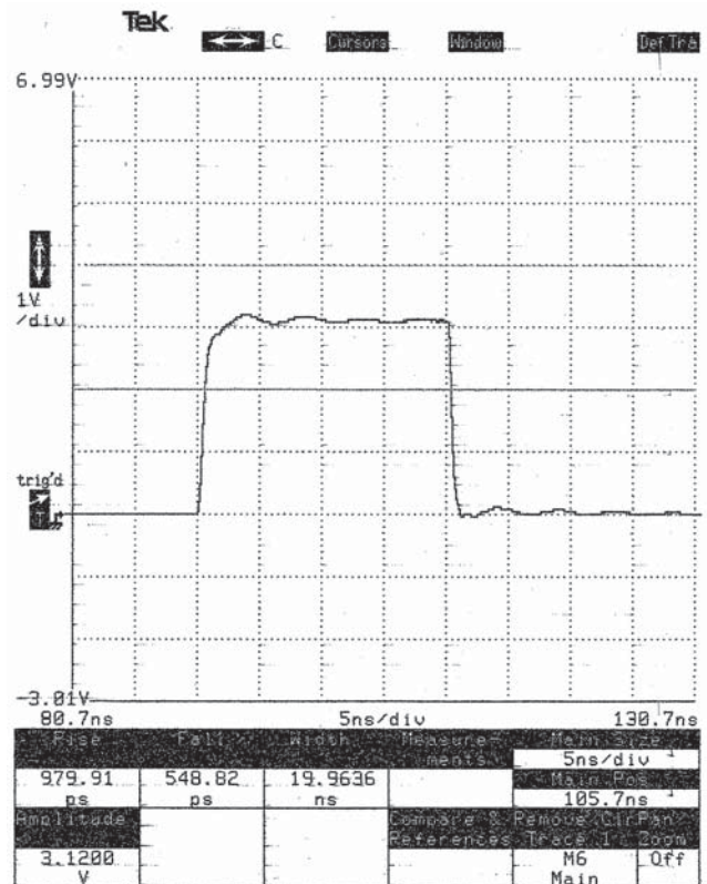
J730-22, -31 Driving 50 \Omega Load
