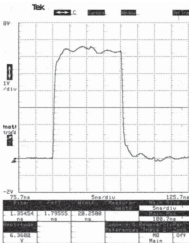
J730-22, -31 Driving Hi-Z Load
