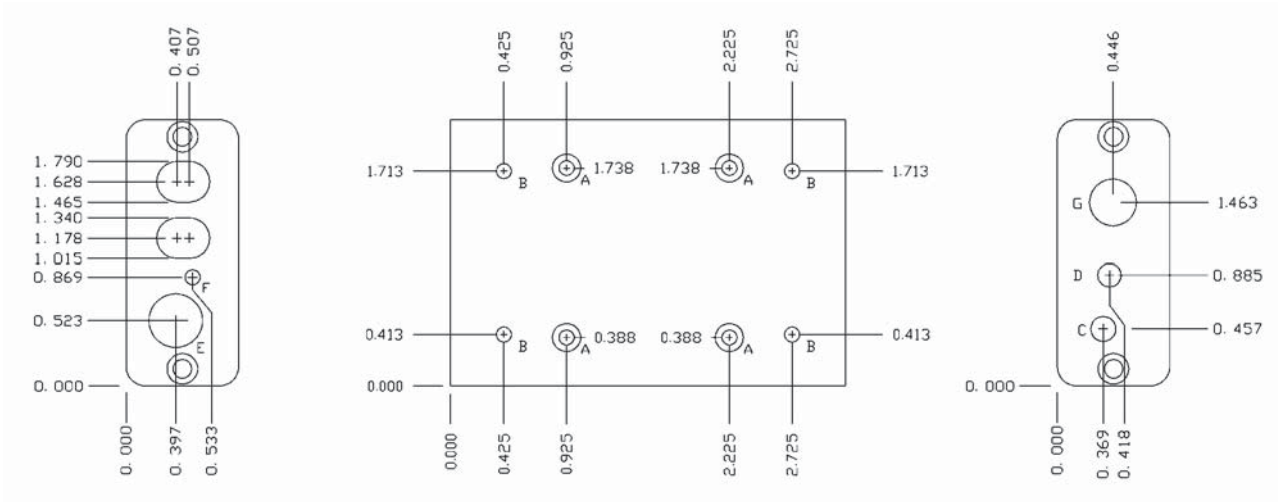
Figure 5. J730 Mounting Dimensions
